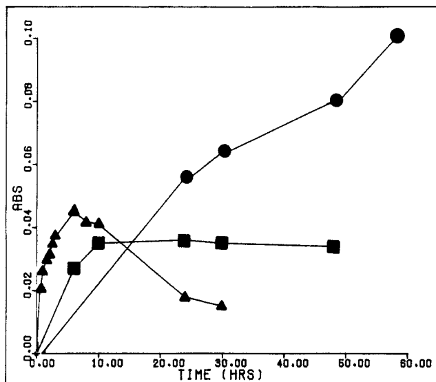
Figure 1. Absorptions for \text{Fe}_3(\text{CO})_{11}\text{P}(\text{OPh})_3 (▲), \text{Fe}_3(\text{CO})_{10}(\text{P}(\text{OPh})_3)_2 (■), and \text{Fe}_3(\text{CO})_9(\text{P}(\text{OPh})_3)_3 (●) during the reaction of \text{P}(\text{OPh})_3 with \text{Fe}_3(\text{CO})_{12} at 30 °C in hexane. The pattern is typical for consecutive substitution reactions.
