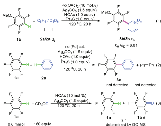
Scheme 2. Mechanism Investigation
