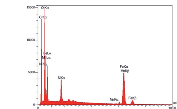
Fig. 3 EDX image of \text{Fe}_3\text{O}_4\text{@NFC@NNSM-Mn(III)} .
