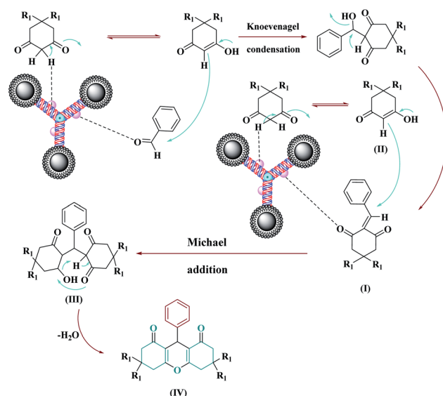
Scheme 3 A plausible mechanism for the synthesis of xanthene while using the \text{Fe}_3\text{O}_4\text{@NFC@NNSM-Mn(III)} catalyst.
