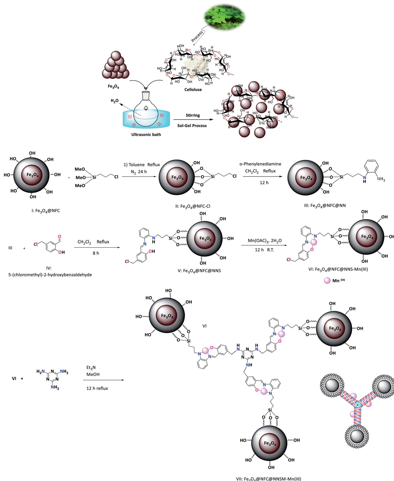
Scheme 1 Overall flowchart for the fabrication of \text{Fe}_3\text{O}_4@NFC@NNSM-Mn(III) .
