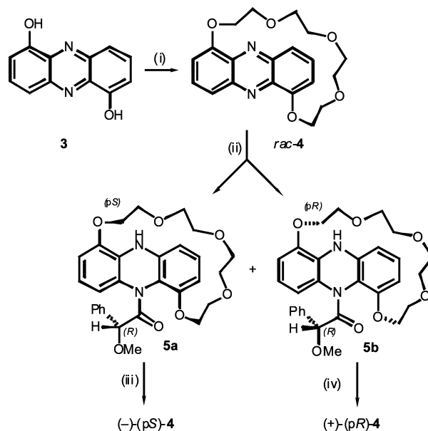
Scheme 2 Reagents and conditions: (i) \text{I}[\text{CH}_2\text{CH}_2\text{O}]_3\text{CH}_2\text{CH}_2\text{I} , \text{K}_2\text{CO}_3 , DMF, 80^\circ\text{C} , 30 h, 14%; (ii) \text{H}_2 (balloon), 10% Pd-C, \text{CH}_2\text{Cl}_2 , 20^\circ\text{C} , 30 min; then ( R )- \alpha -methoxyphenylacetyl chloride (3.1 equiv.), pyridine (3.8 equiv.), 14% for 5a and 19% for 5b ; (iii) 1.3 M HCl, EtOH– \text{H}_2\text{O} (2 : 1), reflux, 3 d, 31%; (iv) 6.7 M HCl, EtOH– \text{H}_2\text{O} (2 : 1), reflux, 7 d, 34%.
