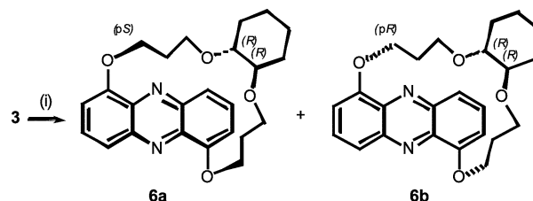
Scheme 3 Reagents and conditions: (i) ( R,R )-1,2-bis(3-iodopropoxy)-cyclohexane, \text{K}_2\text{CO}_3 , DMF, 80^\circ\text{C} , 30 h, 5% for 6a and 5% for 6b .
