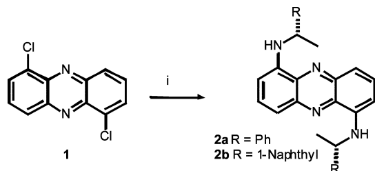
Scheme 1 Reagents and conditions: (i) \text{RCH(Me)NH}_2 (2.2 equiv.), t\text{-BuONa} (2.4 equiv.), \text{Pd}_2(\text{dba})_3 (2 mol%), ( R )-(–)-BINAP (5 mol%), toluene, 99% ( R = Ph) or 55% ( R = 1-naphthyl).
