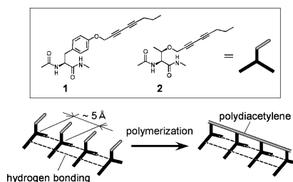
Figure 2. Chemical structures of peptides 1 and 2 (above) and schematic representation of polymerization of the peptide (below).
