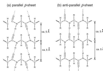
Figure 1. Structural models of parallel (a) and anti -parallel (b) \beta -sheets.
