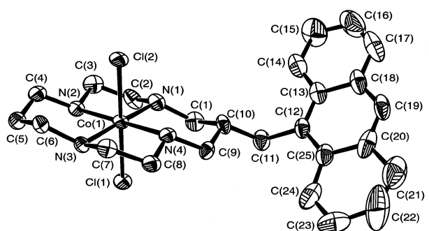
Fig. 2 Diagram of the cation in the crystal structure of trans -[Co(3) 12 ] Cl ·4H 2 O. Ellipsoids are scaled to encompass electron density at the 35% probability level. Hydrogen atoms have been omitted.
