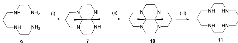
Scheme 2 Reagents and conditions: (i) \text{MeCOCOMe} , \text{CH}_3\text{CN} , -7^\circ\text{C} , 2 h; (ii) \text{BrCH}_2\text{CH}_2\text{Br} , \text{K}_2\text{CO}_3 , \text{CH}_3\text{CN} , 60^\circ\text{C} , 6 h; (iii) HCl, EtOH, 60^\circ\text{C} , 48 h.
