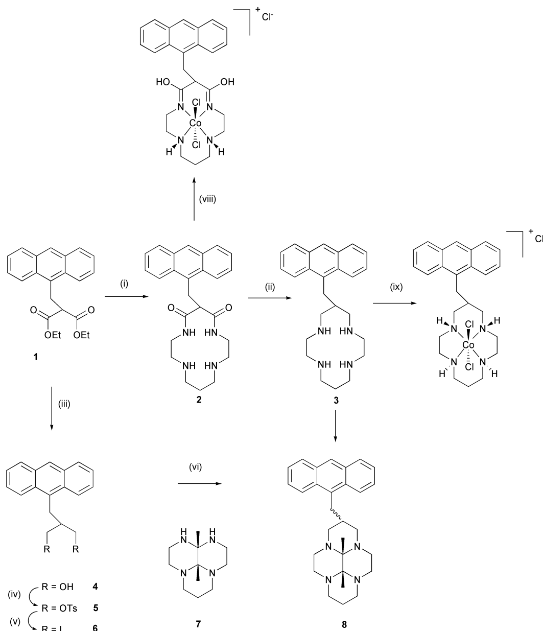
Scheme 1 Reagents and conditions: (i) 2,3,2-tet, EtOH; (ii) \text{BH}_3 \cdot \text{SMe}_2 , THF; (iii) \text{LiAlH}_4 , \text{Et}_2\text{O} ; (iv) TsCl, pyridine; (v) NaI, acetone; (vi) reagent 7 , \text{K}_2\text{CO}_3 , MeCN; (vii) aq. HCl, EtOH; (viii) \text{CoCl}_2 \cdot 6\text{H}_2\text{O} , EtOH, air, then HCl; (ix) \text{CoCl}_2 \cdot 6\text{H}_2\text{O} , NaOH, air, then HCl.
