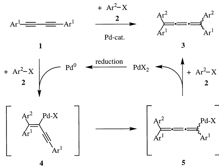
Scheme 1. Mechanistic pathway for the formation of butatriene 3 from butadiyne
