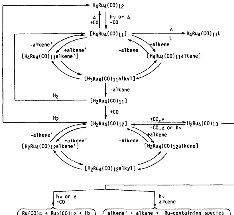
Fig. 3. Representation of possible mechanisms for alkene isomerization, \text{alkene} \leftrightarrow \text{alkene}' , and alkene reduction to form alkane. A similar set of mechanisms could be written for the isomerization employing \pi -allyl hydride intermediates instead of the alkyl. The alkyl intermediates, however, would best account for the formation of alkane.
