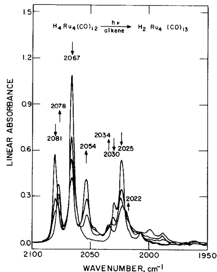
Fig. 1. Infrared spectral changes accompanying near-UV (355 nm) irradiation of [\text{H}_4\text{Ru}_4(\text{CO})_{12}] ( \sim 5 \times 10^{-4} M ) in the presence of 1-pentene ( \sim 10^{-1} M ) in isooctane at 25 °C. Bands at 2081, 2067, 2030, 2025, and 2008 \text{cm}^{-1} are due to [\text{H}_4\text{Ru}_4(\text{CO})_{12}] and those growing with irradiation at 2078, 2066, 2054, 2034, and 2022 \text{cm}^{-1} are due to [\text{H}_2\text{Ru}_4(\text{CO})_{13}] .
