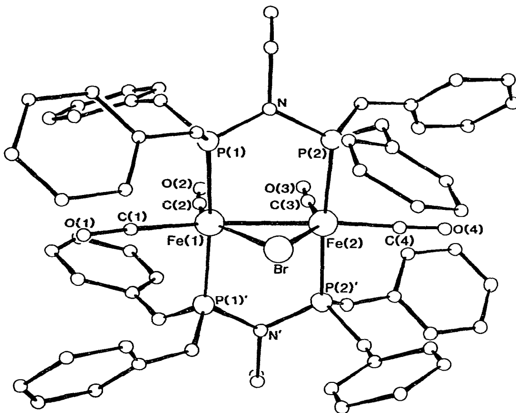
Fig. 1. The molecular structure of [\text{Fe}_2(\mu\text{-Br})(\text{CO})_4\{\mu\text{-(PhO)}_2\text{PN(Et)P(OPh)}_2\}_2] . Hydrogen atoms were not located. Bond lengths: \text{Fe(1)-Fe(2)} , 2.725(5); \text{Fe(1)-Br} , 2.391(4); \text{Fe(2)-Br} , 2.363(5); \text{Fe(1)-P(1)} , 2.235(5); \text{Fe(2)-P(2)} , 2.208(5); \text{Fe(1)-C(1)} , 1.89(3); \text{Fe(1)-C(2)} , 1.69(3); \text{Fe(2)-C(3)} , 1.76(4); \text{Fe(2)-C(4)} , 1.77(3) Å. Bond angles: \text{Fe(1)-Br-Fe(2)} , 69.9(1); \text{Fe(2)-Fe(1)-P(1)} , 91.7(2); \text{Fe(1)-Fe(2)-P(2)} , 92.0(2); \text{Fe(2)-Fe(1)-C(1)} , 167(1); \text{Fe(2)-Fe(1)-C(2)} , 93(1); \text{Fe(1)-Fe(2)-C(3)} , 89(1); \text{Fe(1)-Fe(2)-C(4)} , 167(1)°.
