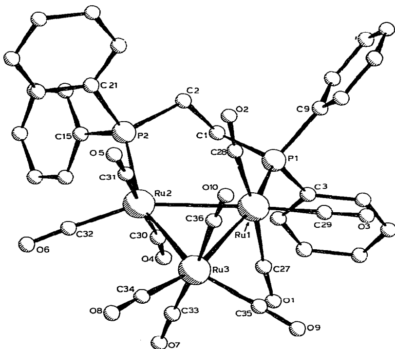
Fig. 1. PLUTO plot of the molecular structure of \text{Ru}_3(\text{CO})_{10}(\text{dppe}) (2).
