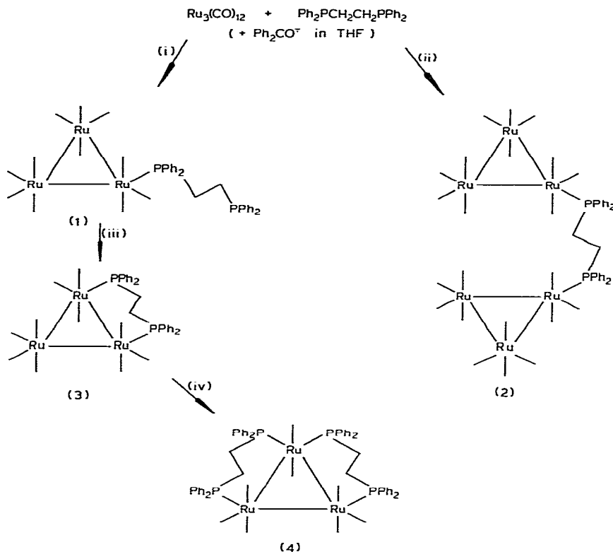
SCHEME 1. Reactions of \text{Ru}_3(\text{CO})_{12} and dppe. Conditions (i) \text{Ru}_3/\text{dppe} = 1/1 , 40^\circ\text{C} , minimum catalyst, 5 min; (ii) \text{Ru}_3/\text{dppe} = 2/1 , 40^\circ\text{C} ; (iii) \text{Ru}_3/\text{dppe} = 1/1 , 40^\circ\text{C} , excess catalyst, 10 min; (iv) \text{Ru}_3/\text{dppe} = 1/2 , 25^\circ\text{C} , excess catalyst, 15 min.
