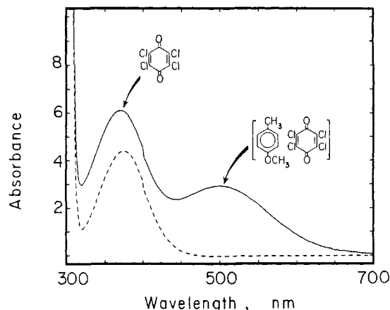
Figure 1. Absorption spectra of 2.0 \times 10^{-3} M CA alone (---) and with 0.4 M MT (—) in dichloromethane.
