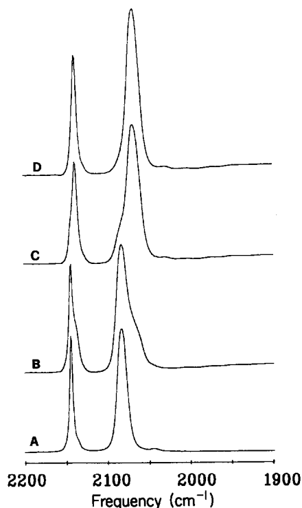
Fig. 2. Infrared spectra in the \nu(\text{CO}) region. Reaction of [\{\text{Ru}(\text{CO})_3\text{Cl}_2\}_2] with \text{Et}_3\text{SiOH} in \text{CH}_2\text{Cl}_2 : (A) [\{\text{Ru}(\text{CO})_3\text{Cl}_2\}_2] in \text{CH}_2\text{Cl}_2 ; (B) 2 min after addition of \text{Et}_3\text{SiOH} ; (C) after a further 30 min; (D) after a further 45 min.
