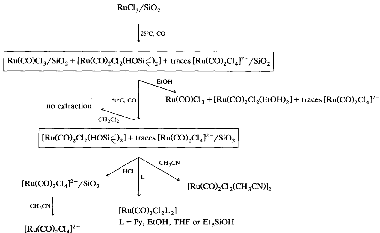
Scheme 1.
