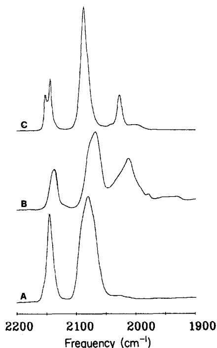
Fig. 3. Infrared spectra in the \nu(\text{CO}) region. Reactivity of physisorbed [\{\text{Ru}(\text{CO})_3\text{Cl}_2\}_2] under \text{CO} + \text{H}_2\text{O} : (A) physisorbed [\{\text{Ru}(\text{CO})_3\text{Cl}_2\}_2] ; (B) after 3 days at 100^\circ\text{C} ; (C) species extracted with \text{CH}_2\text{Cl}_2 .
