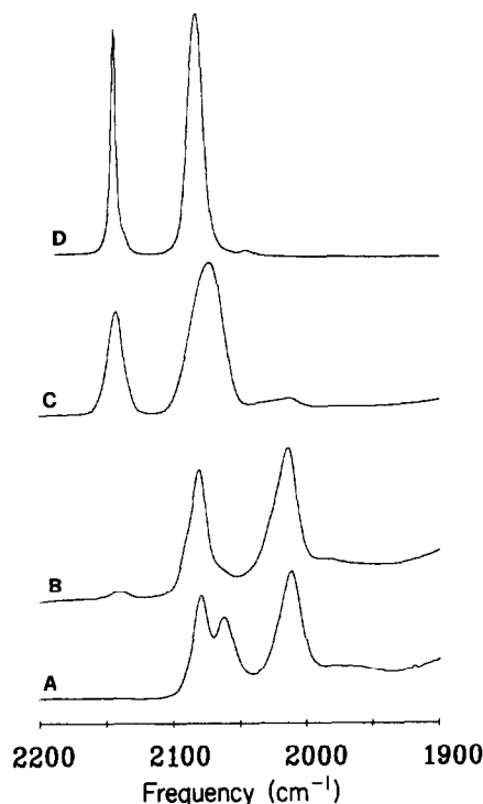
Fig. 1. Infrared spectra in the \nu(\text{CO}) region. Reactivity of physisorbed \text{RuCl}_3/\text{SiO}_2 under CO: (A) after 3 days at 25^\circ\text{C} ; (B) a further 4 days at 50^\circ\text{C} ; (C) a further 2 days at 100^\circ\text{C} ; (D) recrystallized [\{\text{Ru}(\text{CO})_3\text{Cl}_2\}_2] in \text{CH}_2\text{Cl}_2 .
