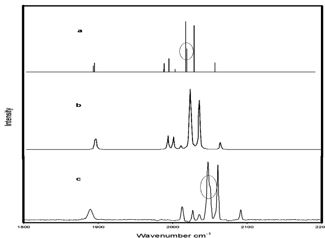
Figure 1. DFT-predicted spectrum of (\mu_4\text{-}\eta^2\text{-2-butyne})\text{Rh}_4(\text{CO})_8(\mu\text{-CO})_2 using (a) GaussView03 and (b) Molden43 and the (c) high-resolution experimental spectrum of (\mu_4\text{-}\eta^2\text{-3-hexyne})\text{Rh}_4(\text{CO})_8(\mu\text{-CO})_2 .
