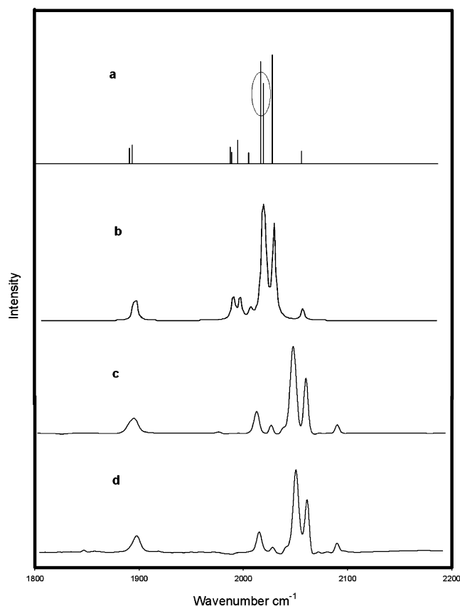
Figure 3. DFT-predicted spectrum of (\mu_4\text{-}\eta^2\text{-propyne})\text{Rh}_4(\text{CO})_8(\mu\text{-CO})_2 using (a) GaussView03 and (b) Molden43 and the low-resolution experimental spectra of (c) (\mu_4\text{-}\eta^2\text{-1-heptyne})\text{Rh}_4(\text{CO})_8(\mu\text{-CO})_2 and (d) (\mu_4\text{-}\eta^2\text{-phenylacetylene})\text{Rh}_4(\text{CO})_8(\mu\text{-CO})_2 .
