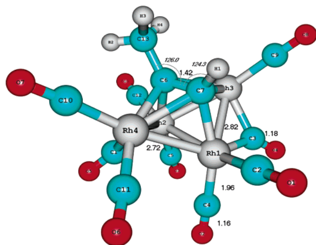
Figure 4. DFT-optimized geometry of \mu_4\text{-}\eta^2\text{-(1-propyne)}\text{Rh}_4(\text{CO})_8(\mu\text{-CO})_2 using PBE/DGDZVP.
