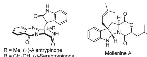
Figure 1. Examples of biologically important molecules containing C γ -tetrasubstituted α-amino acid motifs.
