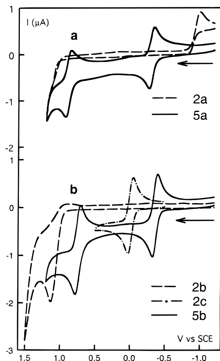
Figure 2. Cyclic voltammograms for (\text{C}_5\text{Me}_5)(\text{dppe})\text{Fe}(\text{C}\equiv\text{CC}\equiv\text{C})\text{Fe}(\text{CO})_2(\text{C}_5\text{R}_5) (a, \text{R} = \text{Ph} ; b, \text{R} = \text{Me} ) and related mononuclear complexes in 0.1 M [\text{nBu}_4\text{N}][\text{PF}_6]/\text{CH}_2\text{Cl}_2 (Pt electrode; V vs SCE; scan rate 0.100 V/s; 20 °C).
