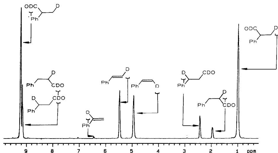
Fig. 3. ^2\text{H} NMR spectrum (46 MHz, 25^\circ\text{C} ) of the crude reaction mixture in benzene obtained by deuteroformylation of styrene at 110^\circ\text{C} and 30% conversion with \text{Rh}_4(\text{CO})_{12} as catalyst.
