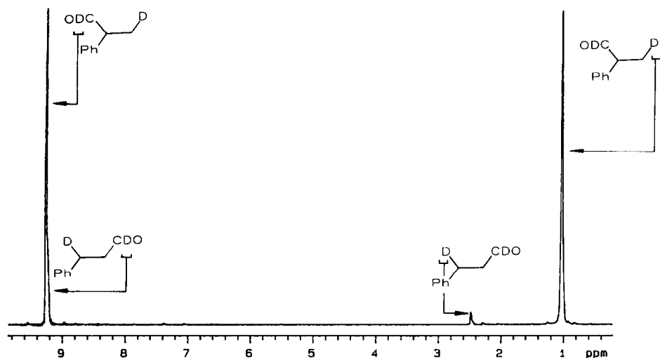
Fig. 2. ^2\text{H} NMR spectrum (46 MHz, 25^\circ\text{C} ) of the crude reaction mixture in benzene obtained by deuteroformylation of styrene at 20^\circ\text{C} and 30% conversion with \text{Rh}_4(\text{CO})_{12} as catalyst.
