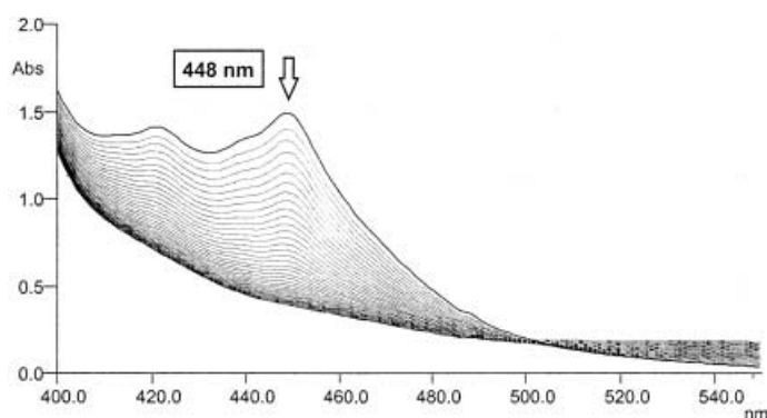
Figure 10. Array of UV/Vis spectra of the reaction of N -phenyldihydrocinotinamide ( 19 ; c = 2.21 \times 10^{-2} M) with p -chloranil ( 1b ; c = 1.05 \times 10^{-3} M) in acetonitrile at 37.0°C.
