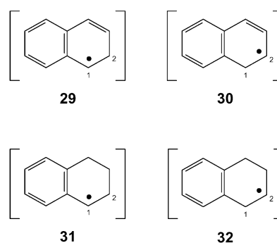
Scheme 6. Potential radical intermediates involved in the quinone oxidation of 1,2-dihydronaphthalene 7 and tetralin 9 .
