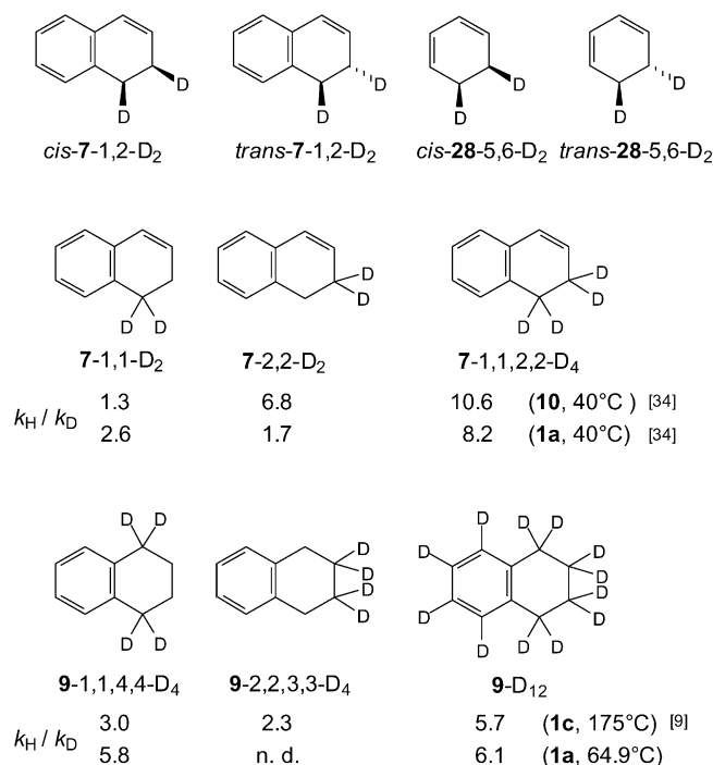
Scheme 5. Specifically deuterated 1,2-dihydronaphthalene, 1,3-cyclohexadiene, and tetralin derivatives used for investigation of the stereochemical course and the kinetic isotope effect of the quinone oxidation of formal 1,3-dienes (n. d. = not determined).
