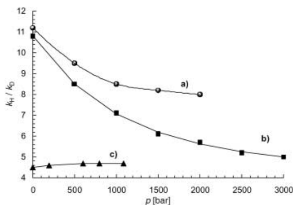
Figure 5. Effect of pressure on the kinetic isotope effect ( k_{\text{H}}/k_{\text{D}} ) of hydrogen transfer reactions: a) reaction of leuco crystal violet with p -chloranil in acetonitrile at 26.5^\circ\text{C} , [31] b) reaction of DDQ ( 1a ) with 5 in MTBE at 25^\circ\text{C} , c) proton transfer from benzoic acid to diphenyldiazomethane at 26.5^\circ\text{C} . [31]
