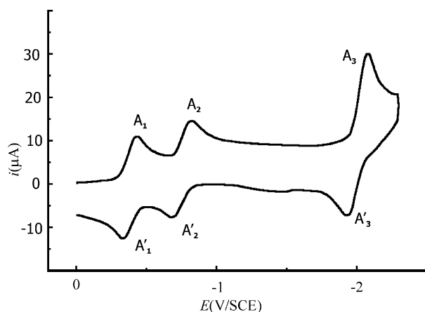
Fig. 5. Cyclic voltammogram of 5 in THF ( 0.2 \text{ mol l}^{-1} of \text{NBu}_4\text{PF}_6 ) on a carbon electrode. Sweep rate: 0.1 \text{ V s}^{-1} . Starting potential: 0 V.
