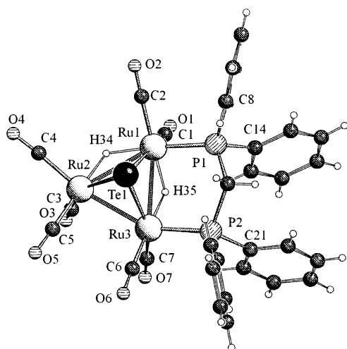
Fig. 3. Molecular structure of [\text{Ru}_3\text{H}_2(\text{CO})_7(\text{dppm})\text{Te}] ( 6 ).
