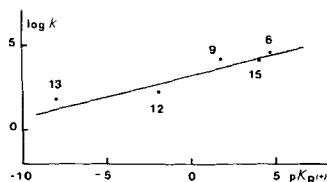
Fig. 5. Plot of \log k for dehydrogenation with DDQ vs. the pK_R^\oplus of the corresponding carbenium ions
