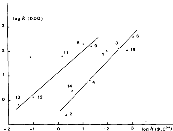
Fig. 1. Rates of dehydrogenation with DDQ vs. triphenylmethylfluoroborate (Data from Table I)
