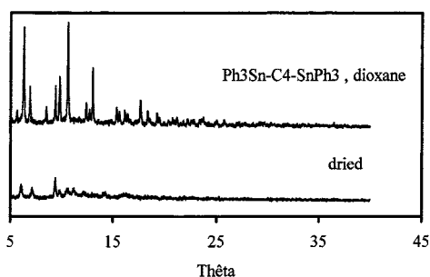
Figure 4. X-ray powder patterns of 4 :dioxane before and after removal of the included solvent molecule.
