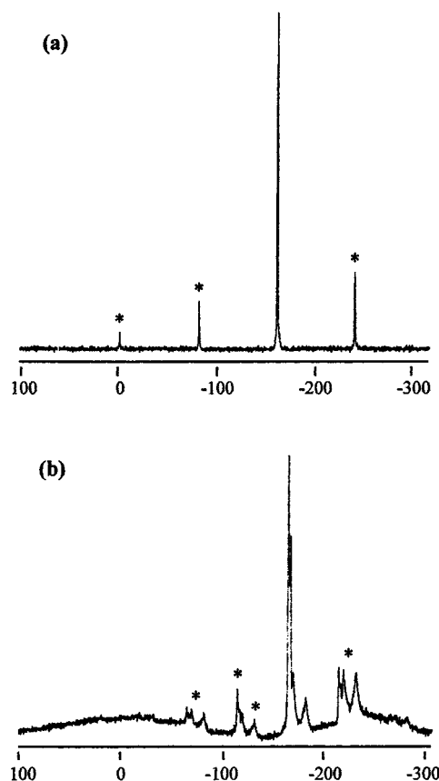
Figure 2. Solid-state ^{119}\text{Sn} MAS NMR spectra of 4 : (a) with included dioxane, observation frequency 149.2 MHz, number of transients 8008, recycle delay time 10 s, 0 Hz line broadening, spinning rate 12 kHz; (b) without included dioxane, observation frequency 74.6 MHz, number of transients 8736, recycle delay time 10 s, 0 Hz line broadening, spinning rate 3.7 kHz. Asterisks denote spinning sidebands.
