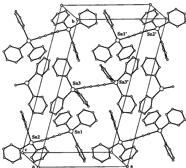
Figure 7. Packing diagram of 4 .
