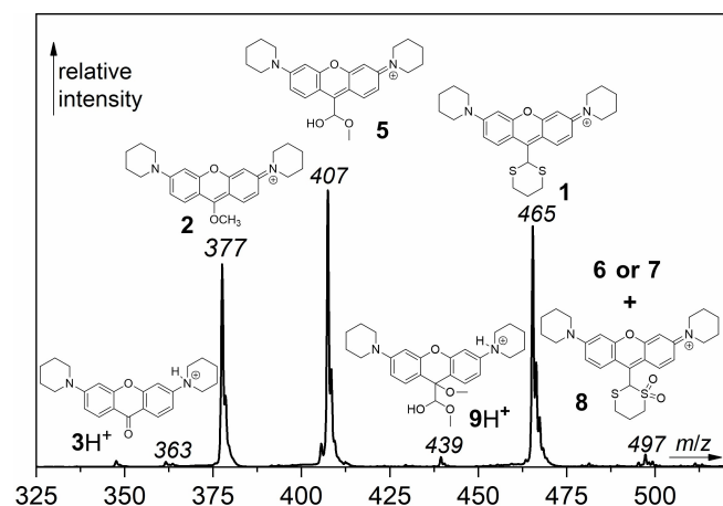
Figure 2. A representative MS spectrum collected after 1 h of irradiation of 1 ( c = 10^{-5} mol dm ^{-3} ) in methanol with LEDs ( \lambda_{\text{irr}} = 592 nm, for the setup see Figures S54 and S55).
