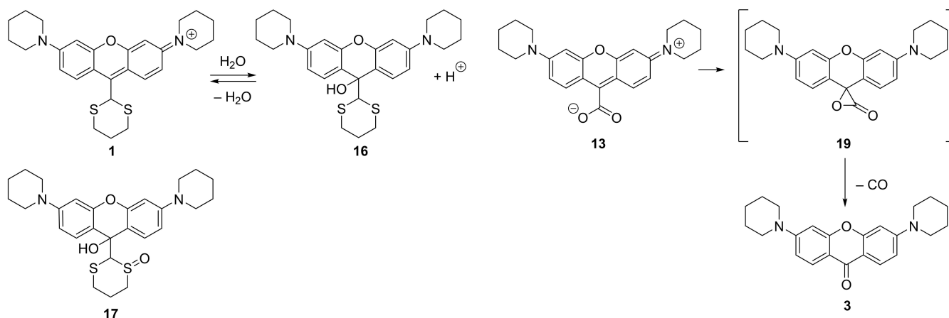
Scheme 4. Equilibrium between 1 and its corresponding xanthrydrol 16 in an aqueous solution, and 17 as the product of oxidation of 1 or 16 .
