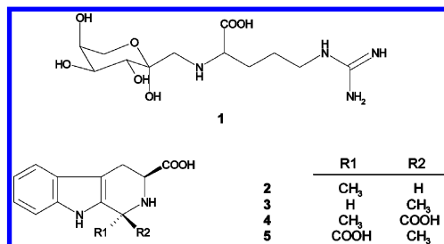
Figure 1. Chemical structures of antioxidants previously identified in aged garlic extract: N \alpha -(1-deoxy-D-fructos-1-yl)-L-arginine (1), (1 R ,3 S )-1-methyl-1,2,3,4-tetrahydro- \beta -carboline-3-carboxylic acid (2), (1 S ,3 S )-1-methyl-1,2,3,4-tetrahydro- \beta -carboline-3-carboxylic acid (3), (1 R ,3 S )-1-methyl-1,2,3,4-tetrahydro- \beta -carboline-1,3-dicarboxylic acid (4), and (1 S ,3 S )-1-methyl-1,2,3,4-tetrahydro- \beta -carboline-1,3-dicarboxylic acid (5).
