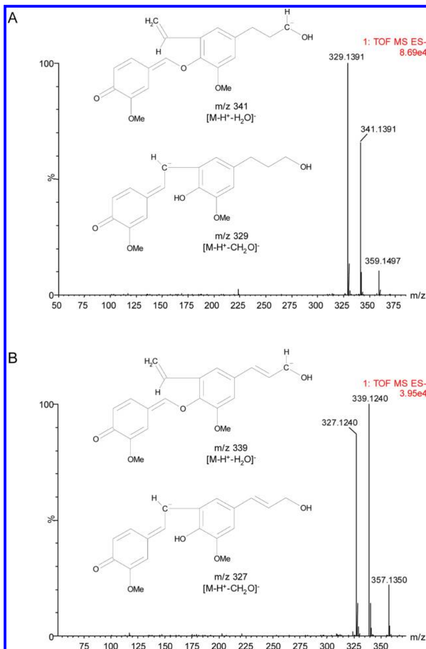
Figure 5. TOF-MS (ESI − ) spectra of (A) (−)-(2R,3S)-dihydrodehydrodiconiferyl alcohol (7) and (B) (+)-(2S,3R)-dehydrodiconiferyl alcohol (8).
