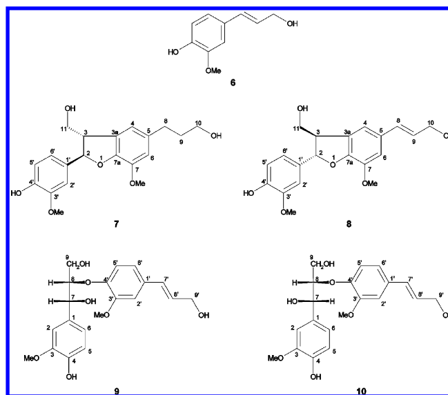
Figure 4. Chemical structures of coniferyl alcohol (6), (–)-(2R,3S)-dihydrodehydrodiconiferyl alcohol (7), (+)-(2S,3R)-dehydrodiconiferyl alcohol (8), erythro -guaiacylglycerol-β-O-4'-coniferyl ether (9), and threo -guaiacylglycerol-β-O-4'-coniferyl ether (10).
