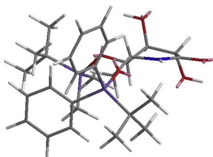
Figure 2. a) 3D model of lactam 11 b) 3D model of lactam 20
