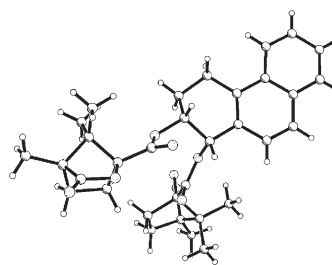
Fig. 1 Crystal structure of one of the two crystallographically independent molecules of (+)- cis -(1 S ,2 R )-1,2,3,4-tetrahydro-phenanthrene dicamphanate 22b cam .
