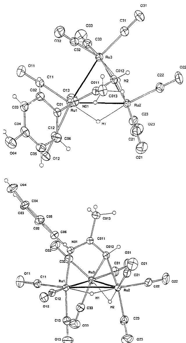
Fig. 1. Molecular structure and atomic labelling scheme for \text{Ru}_3(\mu_3\text{-}\eta^2\text{-(N,C)-4-HOC}_6\text{H}_4\text{N=CMcCH})(\text{CO})_6 \cdot \text{Et}_2\text{O} ( 1 ). 20% thermal ellipsoids are shown for the non-hydrogen atoms; hydrogen atoms have arbitrary radii of 0.1 Å. Projections are shown normal and oblique to the \text{Ru}_3 plane.
