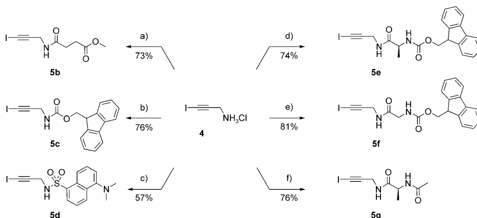
Scheme 2. Derivatization of iodopropargylamine 4 : a) Methyl succinyl chloride, \text{CH}_2\text{Cl}_2 , DIEA, 0^{\circ}\text{C} ; b) Fmoc-L-Ala-OH, \text{CH}_2\text{Cl}_2 , DIEA, 0^{\circ}\text{C} ; c) dansyl chloride, \text{CH}_2\text{Cl}_2 , DIEA, 0^{\circ}\text{C} ; d) Fmoc-L-Ala-OH, PyBOP, \text{CH}_2\text{Cl}_2/\text{DMF} , DIEA, 0^{\circ}\text{C} ; e) Fmoc-Gly-OH, PyBOP, \text{CH}_2\text{Cl}_2/\text{DMF} , DIEA, 0^{\circ}\text{C} ; f) Ac-L-Ala-OH, PyBOP, \text{CH}_2\text{Cl}_2/\text{DMF} , DIEA, 0^{\circ}\text{C} .
