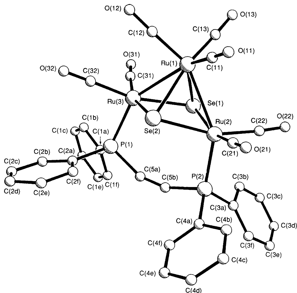
Fig. 2 The molecular structure of [\text{Ru}_3(\mu_3\text{-Se})_2(\text{CO})_7(\text{dppa})] 2
