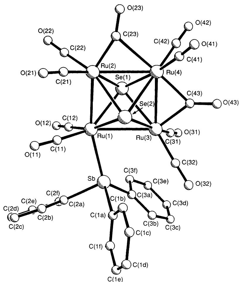
Fig. 3 The molecular structure of [\text{Ru}_4(\mu_4\text{-Se})_2(\text{CO})_{10}(\text{SbPh}_3)] 3
