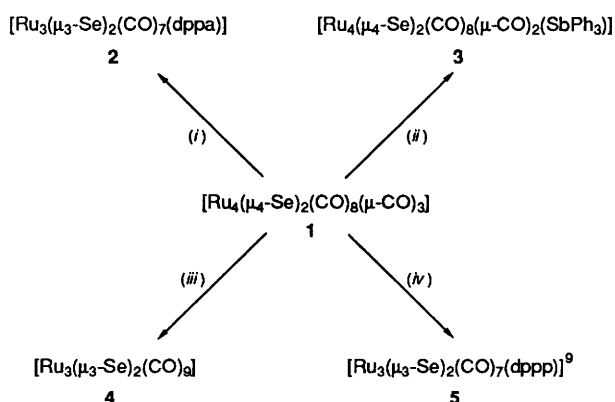
Scheme 1 Summary of the reactivity of [\text{Ru}_4(\mu_4\text{-Se})_2(\text{CO})_8(\mu\text{-CO})_3] 1: (i) +1.0 equivalent dppe in \text{CH}_2\text{Cl}_2 , 25 °C; (ii) +2.0 equivalents \text{Me}_3\text{NO} and 1.5 equivalents \text{SbPh}_3 , \text{CH}_2\text{Cl}_2 , 25 °C; (iii) +CO, 70 atm, \text{CH}_2\text{Cl}_2 , 18 h, 25 °C; (iv) +1.6 equivalents dppe in \text{CH}_2\text{Cl}_2 , 25 °C
