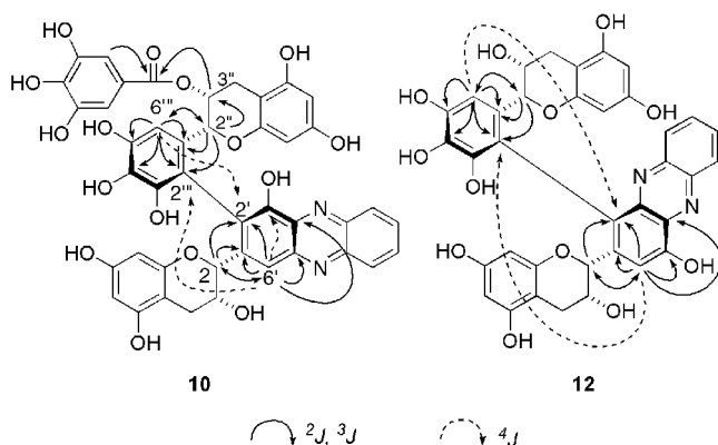
Figure 4. Important HMBC correlations of 10 and 12 .
