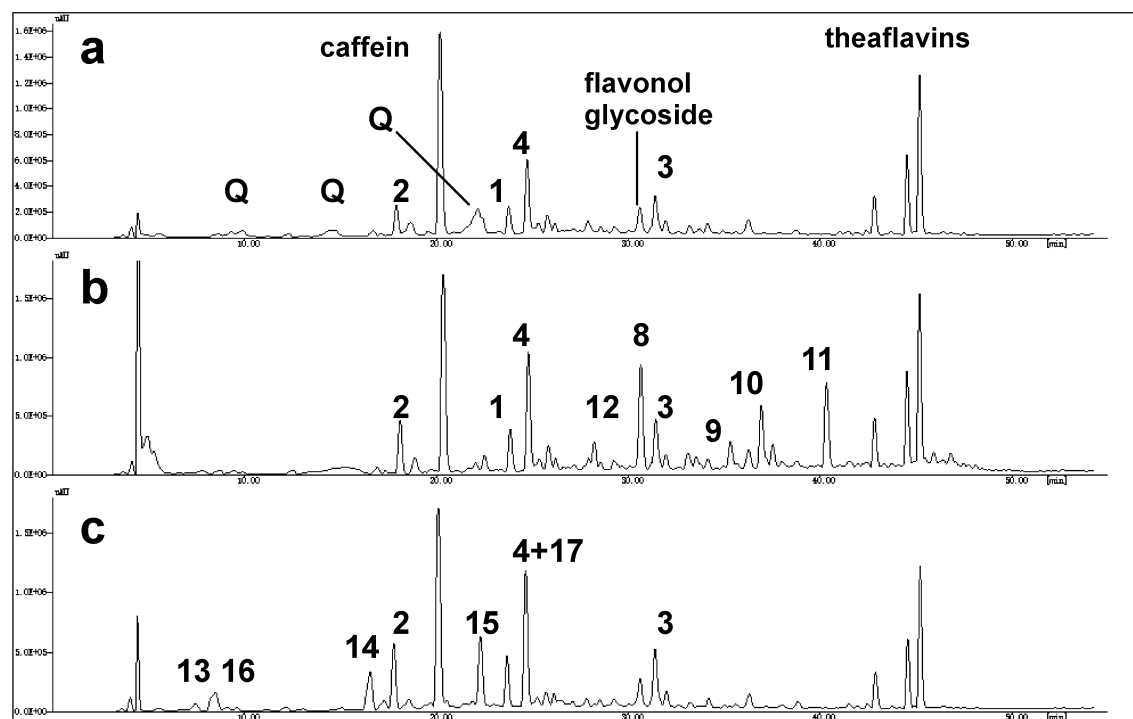
Figure 3. HPLC profiles of fermented tea leaves (UV max. absorbance obtained by photodiodearray detector). (a) Chromatogram of the ethanol extract of fermented tea leaves. (b) Chromatogram of the ethanol extract of fermented tea leaves treated with o -phenylenediamine. The reagent was detected as a large peak at the solvent front. (c) Chromatogram of the ethanol extract of fermented tea leaves heated at 90 °C for 10 min.
