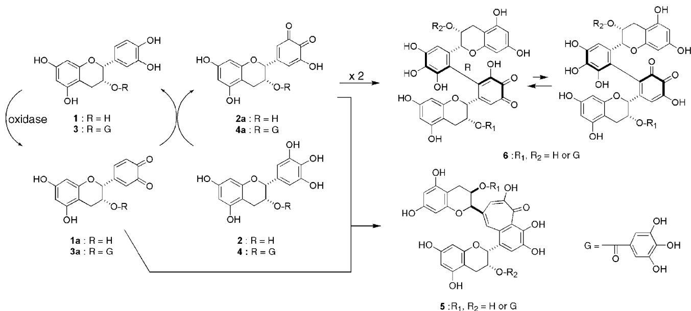
Figure 1. Proposed mechanism for formation of theaflavins and quinone dimers.
