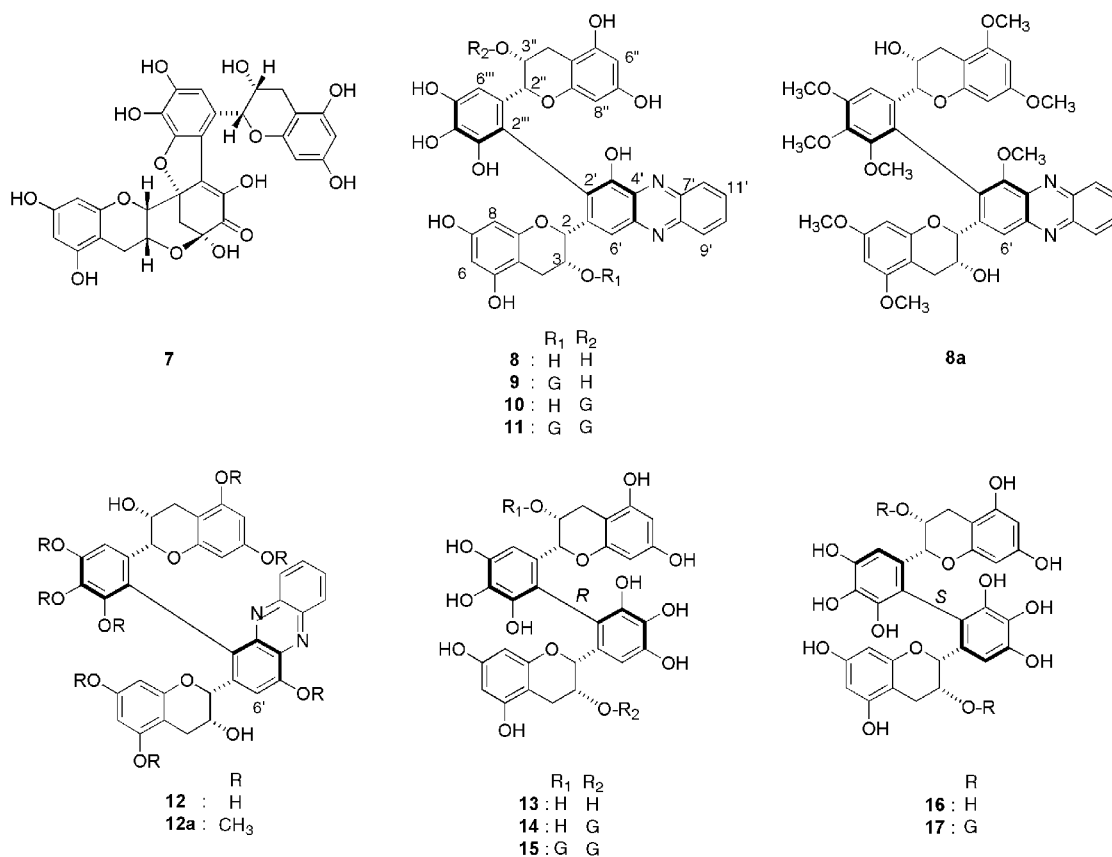
Figure 2. Structures of epigallocatechin oxidation products and phenazine derivatives.
