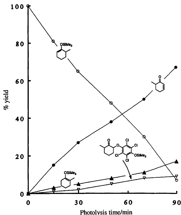
Fig. 4 Oxidative elimination and addition of 6-methylcyclohexenyl trimethylsilyl ether ( 8 ) with photoactivated chloranil, showing the concomitant isomerization to 2-methylcyclohexenyl silyl ether ( 7 )
