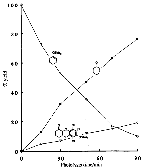
Fig. 3 Time-dependent conversion of cyclohexanone enol trimethylsilyl ether ( 2 ) to cyclohex-2-enone ( 2E ) and adduct ( 2A ) by photoactivated chloranil in dichloromethane at 25 °C
