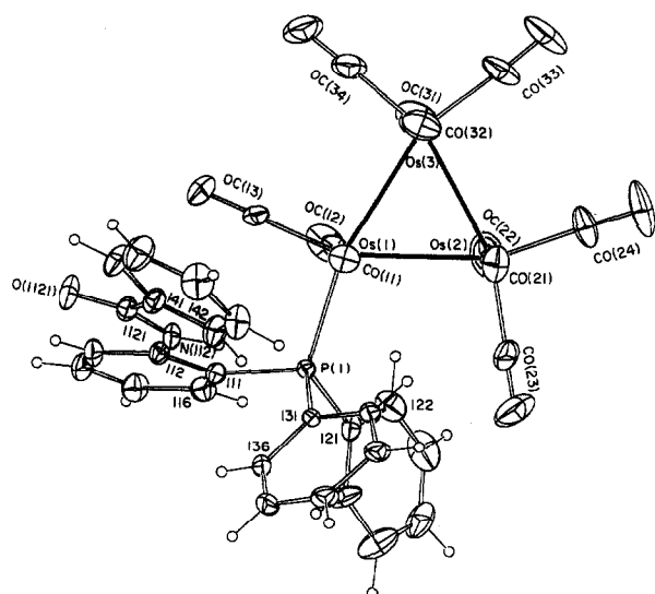
Fig. 2. Plot of a molecule of \text{Os}_3(\text{CO})_{11}[\text{PPh}_2[\text{C}_6\text{H}_4\text{NHC}(\text{O})\text{Ph}-2]] (10).
