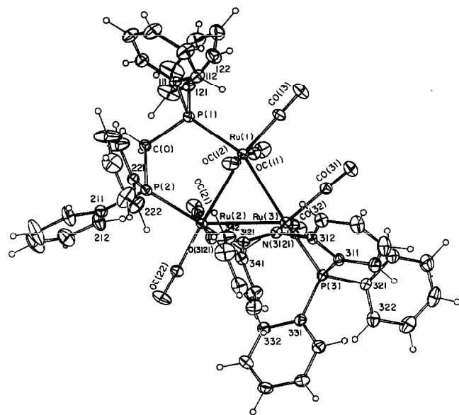
Fig. 9. Plot of a molecule of Ru_3(\mu-H)\{\mu-PPh_2[C_6H_4NC(Ph)O-2]\}(\mu-dppm)(CO)_7 (9).
