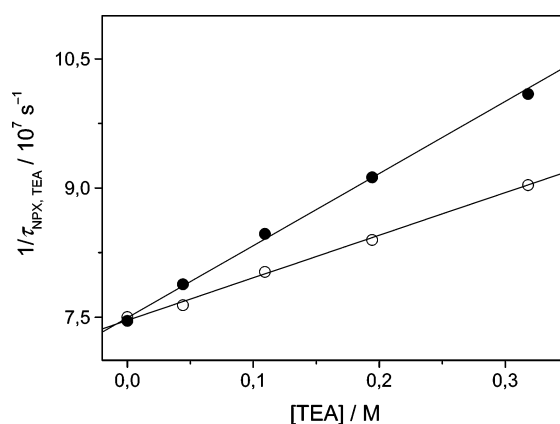
Figure 6. Plots of the inverse lifetime of NPX versus TEA concentration. The data were obtained from time-resolved fluorescence quenching of (S,S)-NPX-NAP (full circles) and (S,R)-NPX-NAP (open circles) by TEA at \lambda_{\text{exc}} = 325 nm in n -hexane.
