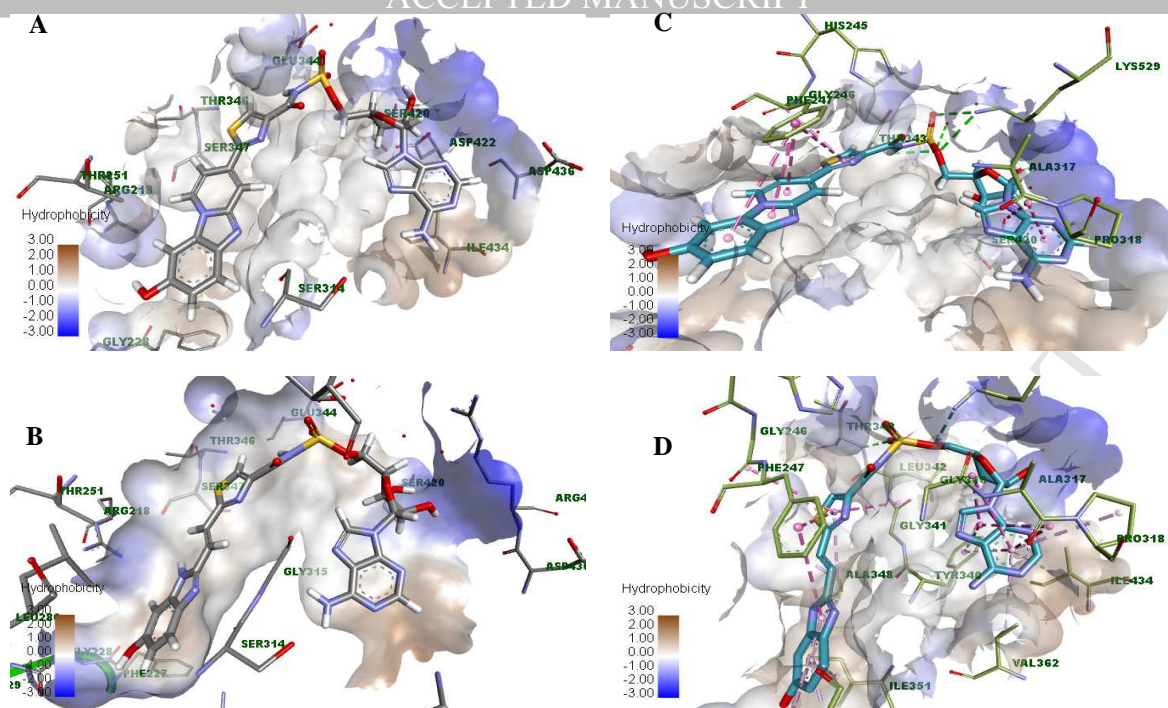
Fig. 1. - A and B - Pose prediction for PBiLH 2 and BiLH 2 in PpyLuc pocket; C and D - PBiLH 2 and BiLH 2 with predicted interactions; Colour code: Pink – Hydrophobic interactions; Green – hydrogen bonds
