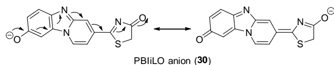
Figure 6. Potential resonance forms of light emitting PBiLH 2 ( 30 ) in
