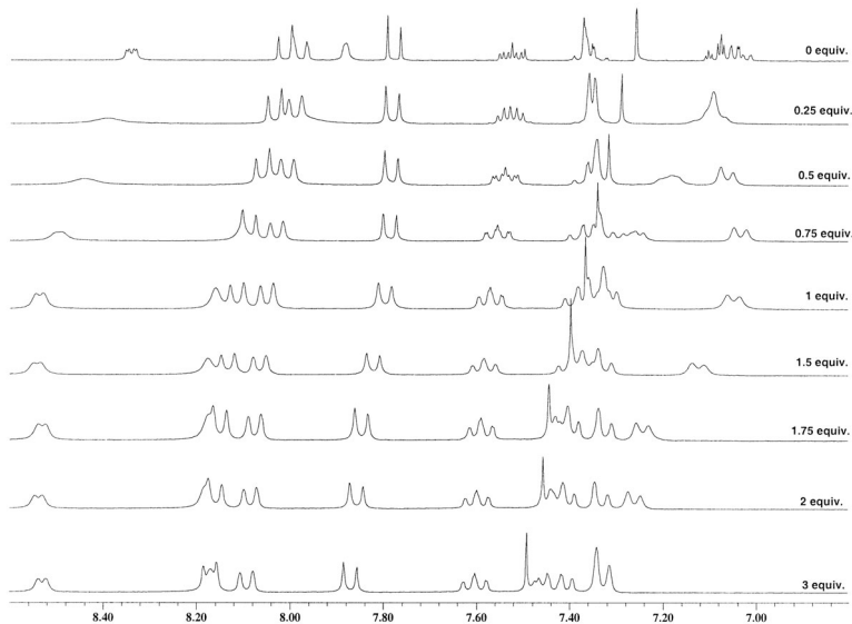
FIG. 2 ^1\text{H} NMR spectra of ( RS )- 8 ( c 0.01 mol/l) after addition of corresponding amounts of \text{ZnCl}_2 , in \text{CDCl}_3\text{--CD}_3\text{CN} mixture (1:1)
