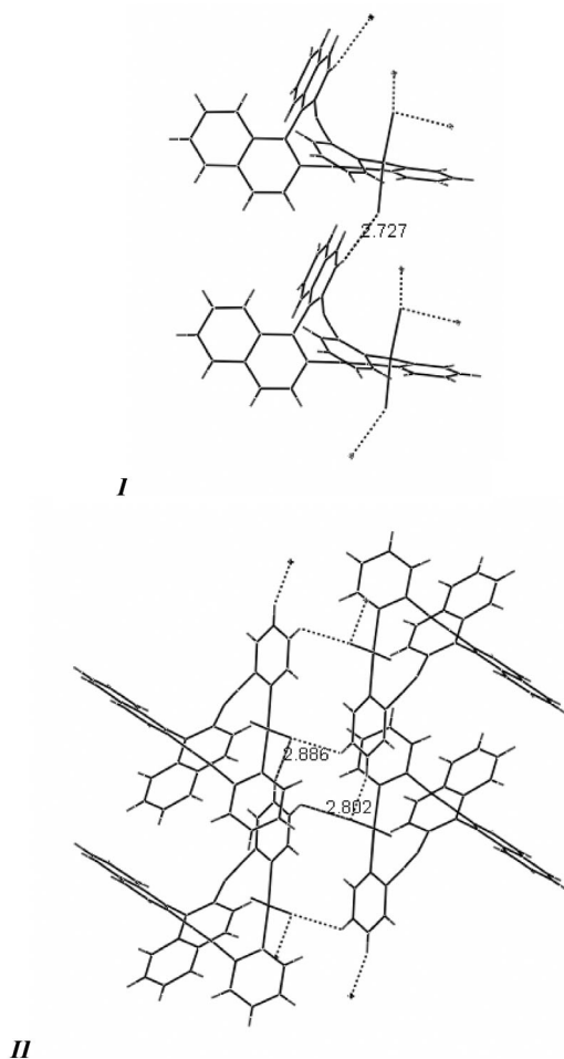
FIG. 6 Schematic representation of supramolecular structure of 17 . Intermolecular short contacts are shown by dotted lines. Solvent molecules are omitted for clarity. I Chain of the homochiral complexes; II two adjacent chains
