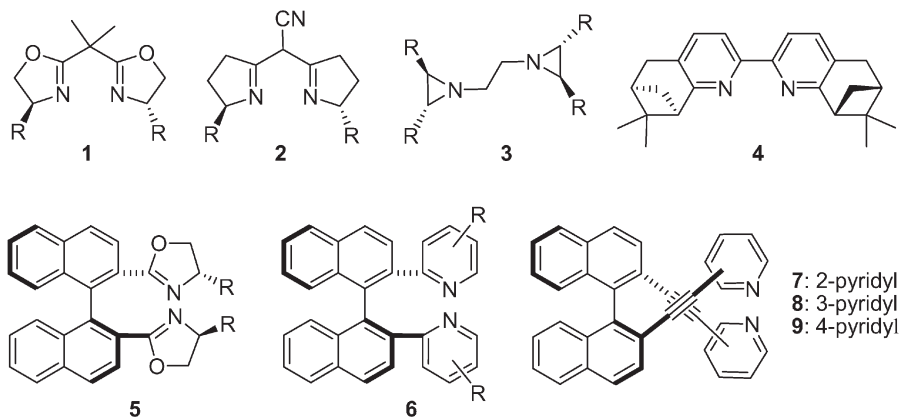
FIG. 1 Selected examples of bidendate N,N -coordinating C_2 -symmetric ligands
