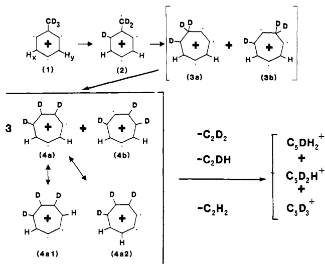
Figure 2. Rearrangement and fragmentation of the tropylium ion analogue of TNT.
