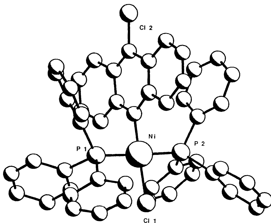
Fig. 1. Molecular structure of \text{Ni}(\text{C}_{14}\text{H}_8\text{Cl})\text{Cl}(\text{PPh}_3)_2 , 11 . Solvent molecules are omitted for simplicity. See footnote on previous page.
