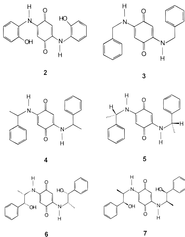
Figure 1. Chemical structures of 2,5-diamino- p -benzoquinones.
