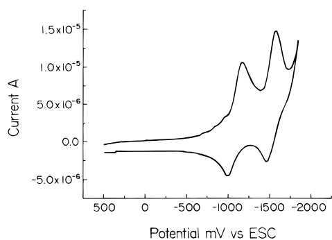
Figure 5. Cyclic voltammogram of 3 mM 2,5-di(α-methylbenzylamine)- p -benzoquinone containing 0.1 M Et_4NBF_4 in CH_3CN (working electrode Pt, reference SCE; scan rate 100 mV/s).
