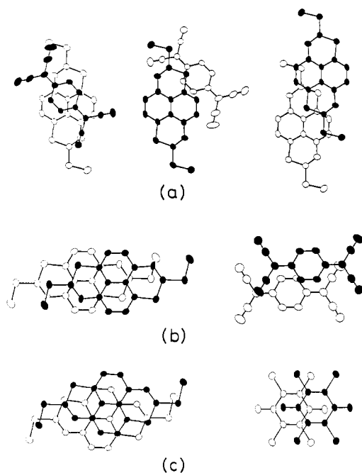
Figure 3. Molecular overlap modes: (a) \alpha -MTDPY-TCNQ; (b) \beta -MTDPY-TCNQ; (c) MTDPY-CHL.
