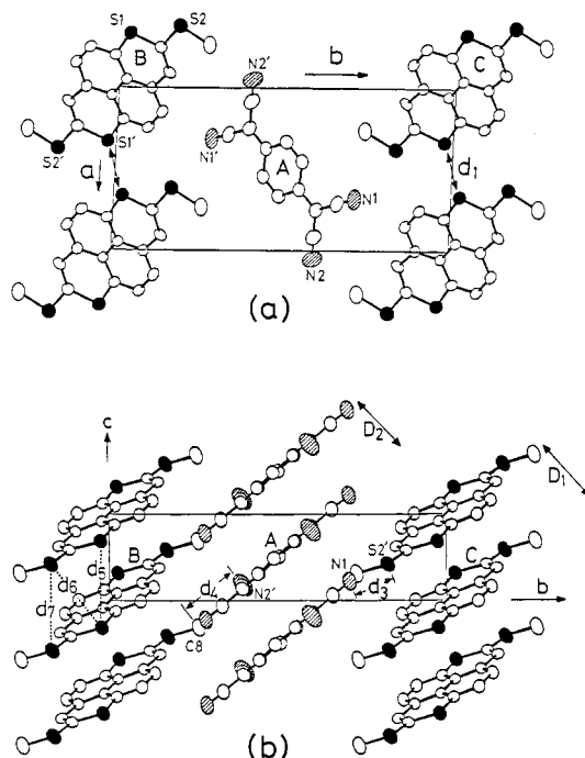
Figure 4. Crystal structures of \beta -MTDPY-TCNQ viewed along (a) the c axis and (b) the a axis. Some distances: d_1 = 3.57 , d_3 = 3.50 , d_4 = 3.28 , d_5 = 4.37 , d_6 = 4.02 , d_7 = 4.37 , D_1 = 3.48 , D_2 = 3.27 Å. For d_2 , see text.
