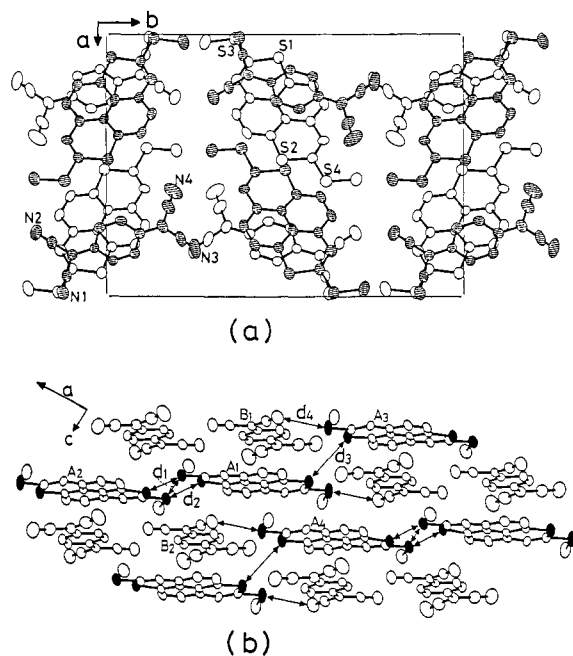
Figure 2. (a) Crystal structure of \alpha -MTDPY-TCNQ viewed along the c axis. (b) View of the donor and acceptor sheet in \alpha -MTDPY-TCNQ. Some distances: d_1 = 3.66 , d_2 = 3.82 , d_3 = 3.93 , d_4 = 3.66 Å.
