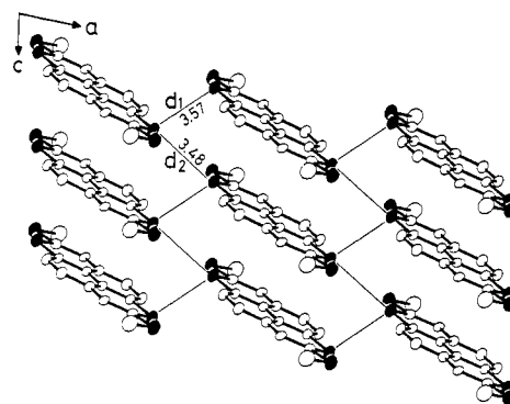
Figure 5. View of the sheet-like network of the donor molecules in \beta -MTDPY-TCNQ.
