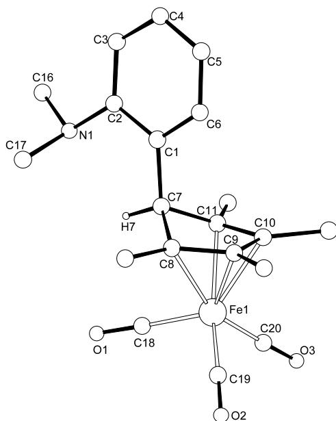
Fig. 2. Solid state structure of 5 . Selected bond lengths (Å) and angles (°): Fe–C8 2.143(2); Fe–C9 2.071(2); Fe–C CO 1.785(2)–1.794(2), C–O 1.143(3)–1.148(2); C7–C8 1.529(2); C8–C9 1.432(2); C9–C10 1.428(3); C10–C11 1.437(2); C11–C7 1.529(2); C7–C1 1.534(2); C7–H7 0.97(2); N1–H7 2.38; C CO –Fe–C CO 93.1(1)–102.3(1).
