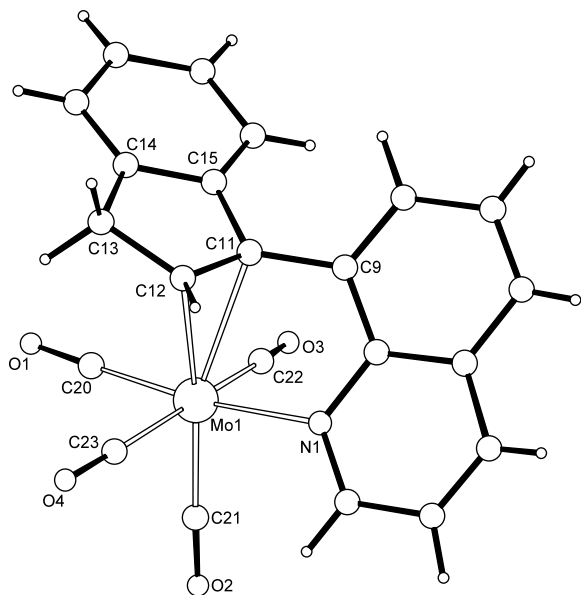
Fig. 5. Solid state structure of 9 . Selected bond lengths (Å) and angles (°): C11–C12 1.396(5), C12–C13 1.523(5), C13–C14 1.504(5), C14–C15 1.402(5), C15–C11 1.483(5), C9–C11 1.490(5), Mo1–C12 2.460(4), Mo1–C11 2.489(4), Mo1–C20 1.967(4), Mo1–C21 1.972(4), Mo1–C22 2.034(4), C20–O1 1.161(4), C21–O2 1.155(5), C22–O3 1.149(4), C23–O4 1.138(5), N1–Mo1–C21 95.9(2), N1–Mo1–C22 95.0(1), N1–Mo1–C23 93.8(2), N1–Mo1–C20 173.1(1).
