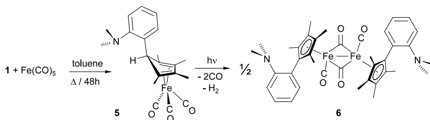
Scheme 2. Formation of the iron complexes 5 and 6 with the ligand 1 . The quinolyl substituted derivative 2 leads directly to the binuclear complex 7 (analogue to 6 ).
