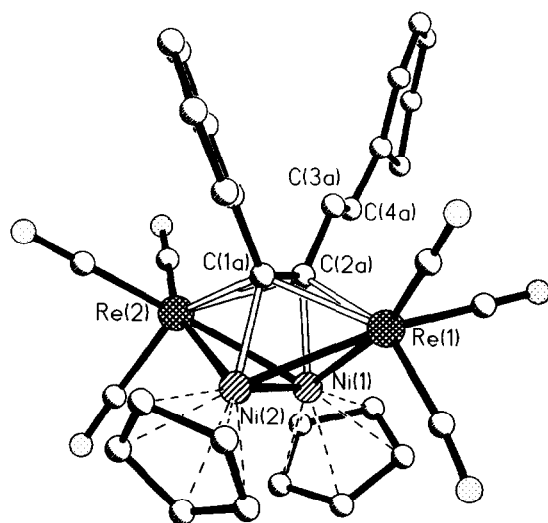
Fig. 2. Molecular structure of \text{Cp}_2\text{Ni}_2\text{Re}_2(\text{CO})_6(\mu_4\text{-PhC}\equiv\text{CCH=CHPh}) .
