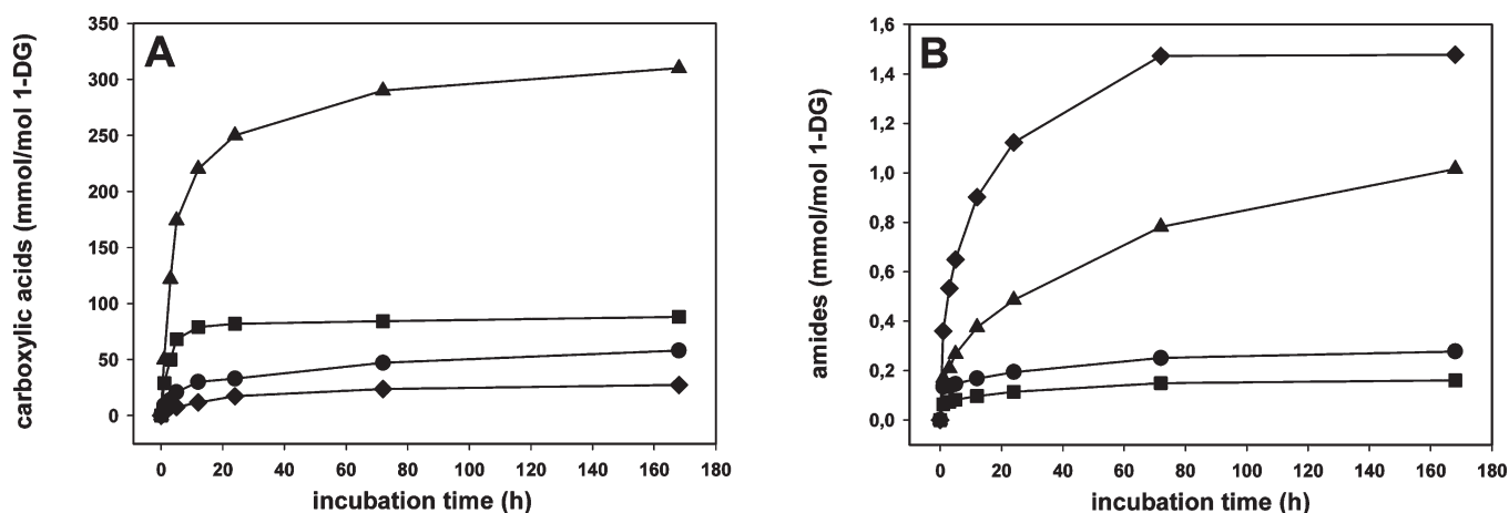
Figure 2. Formation of carboxylic acids ( A ) and corresponding amides ( B ) in 1-DG/ N^\epsilon - t -BOC-lysine incubation mixtures (42 mM in phosphate buffer 0.1 M, pH 7.4, at 37 °C under aerated conditions): acetic acid/ N^\epsilon -acetyl lysine (▲), glyceric acid/ N^\epsilon -glycerinyl lysine (■), lactic acid/ N^\epsilon -lactoyl lysine (●) and formic acid/ N^\epsilon -formyl lysine (◆).
