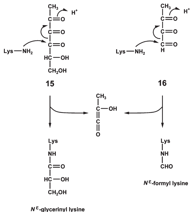
Figure 4. Nucleophilic attack on tricarbons formed by oxidation from 1-DG or 1-DT leads to N^\epsilon -glycerinyl lysine and N^\epsilon -formyl lysine.
