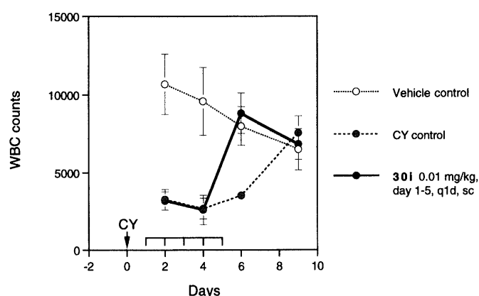
Fig. 3. WBC-Restorative Effect of TAN-1511 Derivatives in the Mouse Leukocytopenia Model
