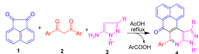
Scheme 1. Synthesis of Pentacyclic Pyrazole-Fused Naphtho-[1,8- fg ]isoquinolines
