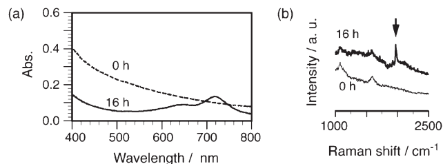
Figure 3. (a) UV-vis spectra of 1 in the presence of SPG before (0 h) and after (16 h) UV irradiation: [\textbf{1}] = 25 \mu\text{g mL}^{-1} , [\text{SPG}] = 25 \mu\text{g mL}^{-1} , aqueous DMSO ( [\text{H}_2\text{O}] = 70 v/v %), and (b) Raman spectra of 1 in the presence of SPG before and after UV irradiation: cast films.
