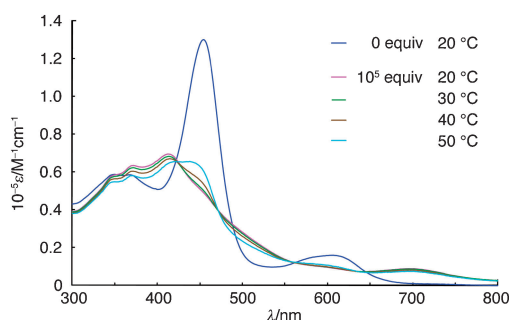
Figure 7. VT-UV-vis spectra of 2a with and without TFA in \text{CHCl}_3 .
