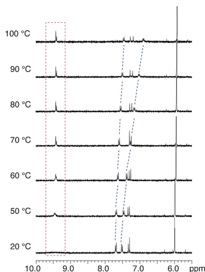
Figure 6. VT- ^1\text{H} NMR spectra of 2a with 25 equiv of TFA- d in \text{C}_2\text{D}_2\text{Cl}_4 (300 MHz). 11
