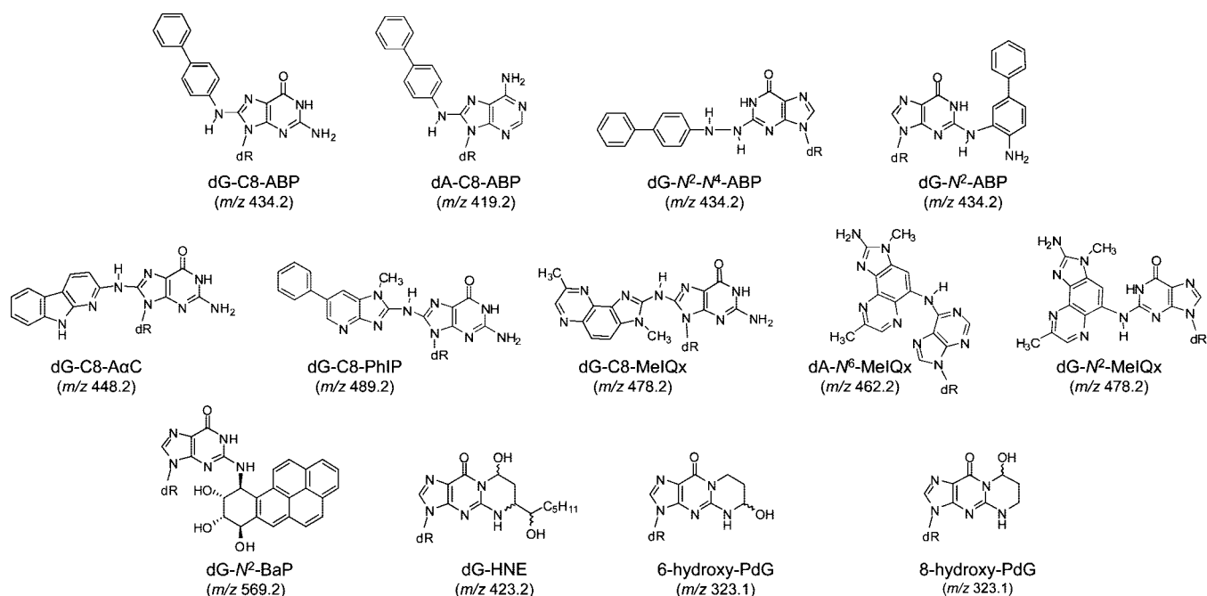
Figure 1. Structures of DNA adducts under investigation.
