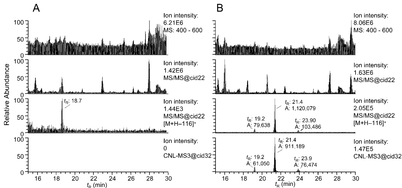
Figure 2. Global CNL-MS 3 data-dependent scanning of 4-ABP adducts in human hepatocytes, either (A) untreated or (B) 4-ABP-treated (10 \mu M). The upper chromatograms in each panel displays the full scan mode from 400 to 600 Da. The second chromatogram down is a collection of all MS/MS spectral chromatograms. The third chromatogram displays all of the peaks that are filtered by the CNL [ M+H ] + \rightarrow [ M+H-116 ] + . The bottom chromatogram displays all of the peaks that were detected by the data-dependent CNL-MS 3 scan mode. The respective t_R and area of response of the ion counts are shown.
