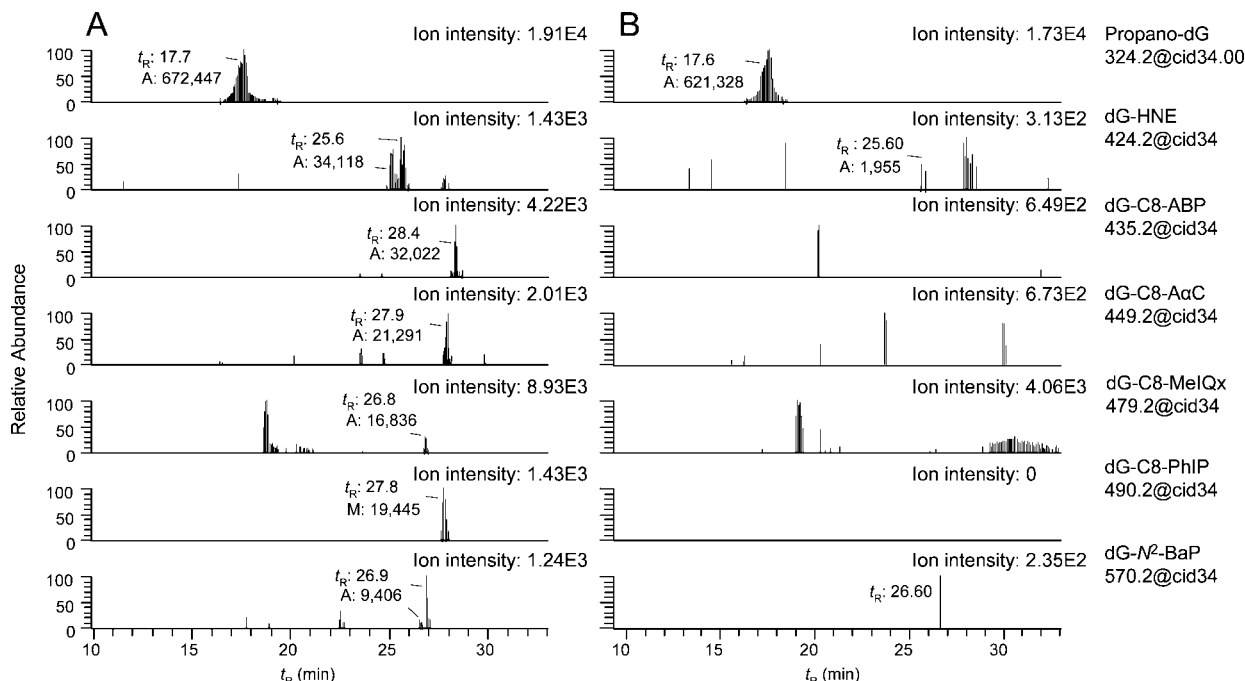
Figure 6. Targeted data-dependent scanning in CNL-MS 3 of DNA adducts in (A) spiked buccal cells and (B) unspiked buccal cells. The chromatograms show the CNL-MS 3 traces for 6-hydroxy-PdG and 8-hydroxy-PdG ( m/z 324.2), dG-HNE ( m/z 424.2), dG-C8-ABP ( m/z 435.2), dG-C8-AαC ( m/z 449.2), dG-C8-MelQx ( m/z 479.2), dG-C8-PhIP ( m/z 490.2), and dG- N 2 -BaP ( m/z 570.2); the area of response of the ion counts are shown.
