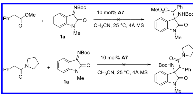
Scheme 1. Control Reaction of Methyl 2-Phenylacetate or Pyrrolidinyl 2-Phenylacetate with 1a
