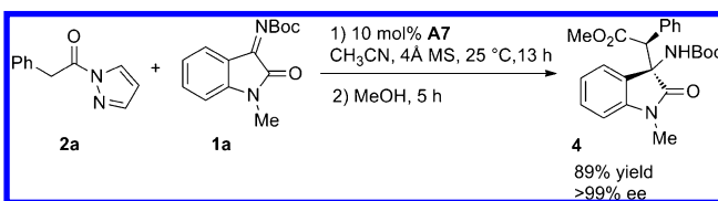
Scheme 2. One-Pot Esterification
