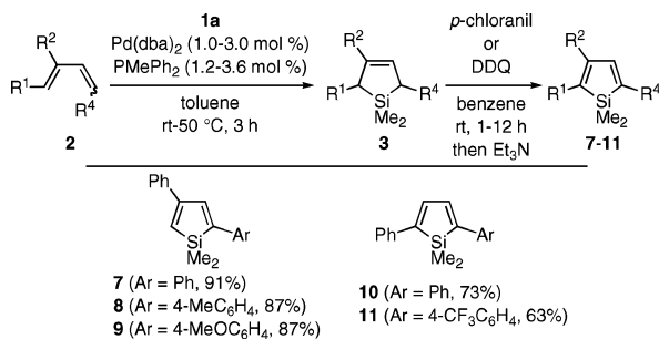
Scheme 1. Synthesis of 2,4- and 2,5-Diarylsiloles from 1,3-Dienes a
