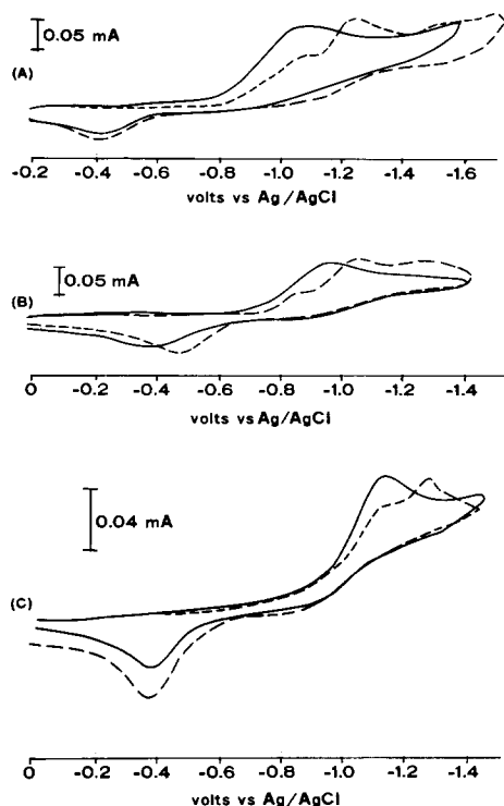
Fig. 7. Cyclic voltammograms of 0.5 mM \text{Ru}_3(\text{CO})_{12} in \text{CH}_2\text{Cl}_2 , 200 \text{ mV s}^{-1} , at Pt, in the absence (—) and presence (-----) of 1.5 M \text{PPh}_3 . (a) acetone; (b) THF; (c) \text{CH}_2\text{Cl}_2 .
