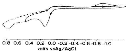
Fig. 8. Cyclic voltammogram of [\text{PPN}][\text{HRu}_3(\text{CO})_{11}] in \text{CH}_2\text{Cl}_2 on Pt, in \text{CH}_2\text{Cl}_2 at 293 K; 200 \text{mV s}^{-1} .
