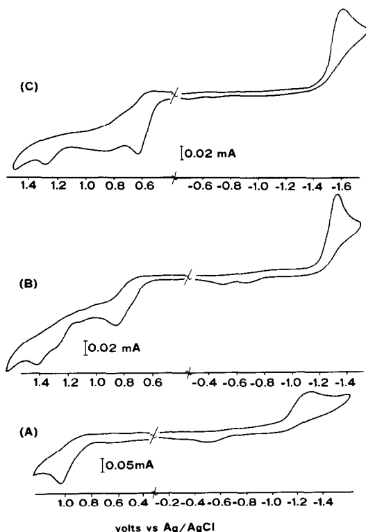
Fig. 5. Cyclic voltammograms in \text{CH}_2\text{Cl}_2 at Pt, 100 \text{ mV s}^{-1} , 293 K under Ar, of (TBAP 0.1 \text{ mol dm}^{-3} ): (a) \text{Ru}_3(\text{CO})_{11}\text{PPh}_3 ; (b) \text{Ru}_3(\text{CO})_{10}(\text{PPh}_3)_2 ; (c) \text{Ru}_3(\text{CO})_9(\text{PPh}_3)_3 .
