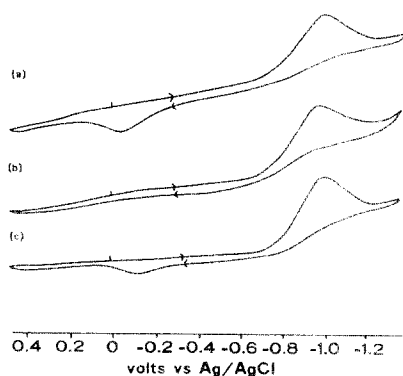
Fig. 3. Cyclic voltammograms of \text{Ru}_3(\text{CO})_{12} in \text{CH}_2\text{Cl}_2 under Ar. (a) [\text{Ru}_3(\text{CO})_{12}] 5 \times 10^{-4} mol \text{dm}^{-3} , 293 K, 200 \text{mV s}^{-1} , Pt, 0.10 mol \text{dm}^{-3} [\text{PPN}][\text{OAc}] . (b) as for (a) except at 253 K. (c) [\text{Ru}_3(\text{CO})_{12}] 5 \times 10^{-4} mol \text{dm}^{-3} , 293 K, 200 \text{mV s}^{-1} , Pt, [\text{PPN}][\text{ClO}_4]/[\text{Bu}_4\text{N}][\text{OH}] , 0.10 mol \text{dm}^{-3}/5 \times 10^{-4} mol \text{dm}^{-3} .
