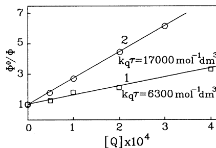
Fig. 3. Stern-Volmer plots on the formation of 1(DPB/AN 1:1 adduct, Q: azulene) and 2(DPB/EVE 1:1 adduct, Q: 9,10-diphenylanthracene).
