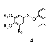
R 1 , R 2 , R 3 = H, Me, Et, Pr, Bu. X = CO, CH 2 =CH 2 CO ( E )
